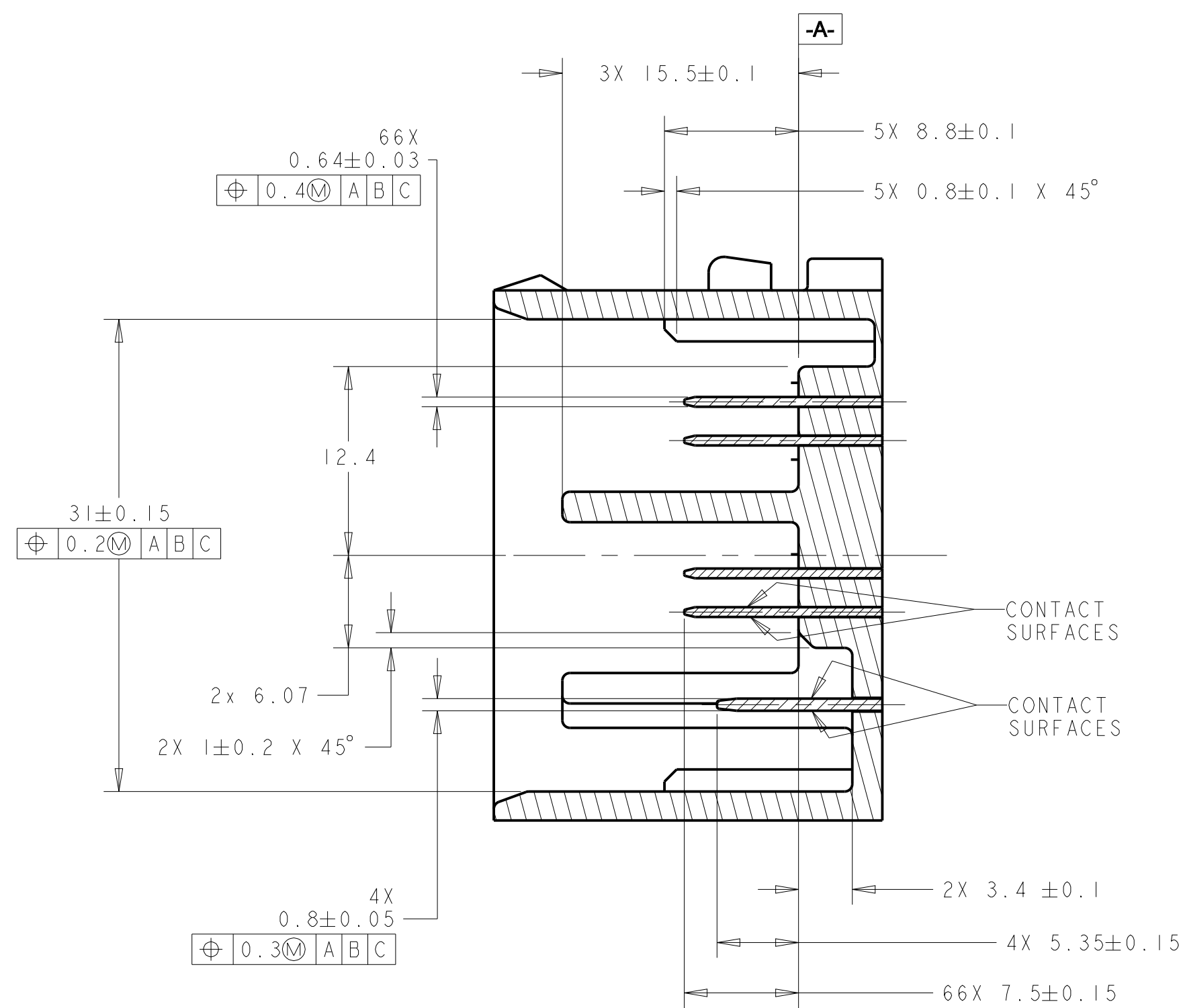
SECTION C-C
