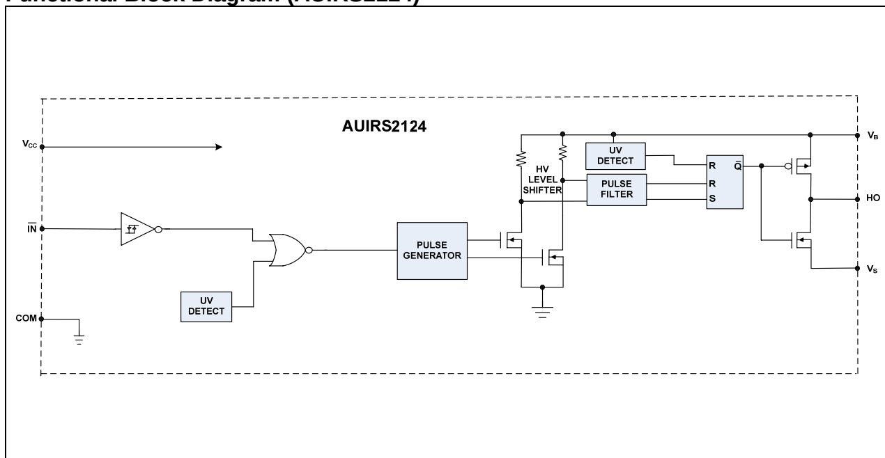
Functional Block Diagram (AUIRS2124)
