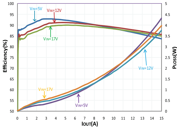
Efficiency/Power Loss vs. Load - P-Save ( V_{DD} = 3.3\text{ V} , V_{OUT} = 1.5\text{ V} , SiC401A)
