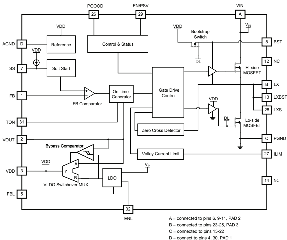
SiC401A/B Functional Block Diagram
