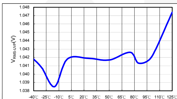
Figure 34. V_{\text{RMS-UVF}} vs. Temperature
