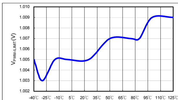
Figure 32. V_{\text{PWM-ILIMIT}} vs. Temperature
