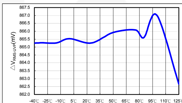
Figure 35. \Delta V_{\text{RMS-UVF}} vs. Temperature
