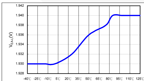
Figure 38. V_{\text{EA-L}} vs. Temperature
