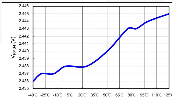
Figure 37. V_{\text{RMS-H}} vs. Temperature
