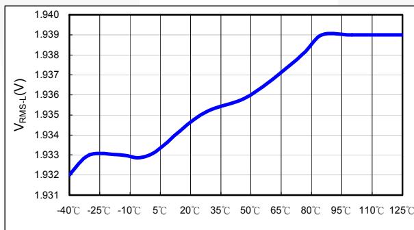
Figure 36. V_{\text{RMS-L}} vs. Temperature
