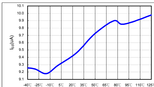
Figure 33. I_{\text{SS}} vs. Temperature
