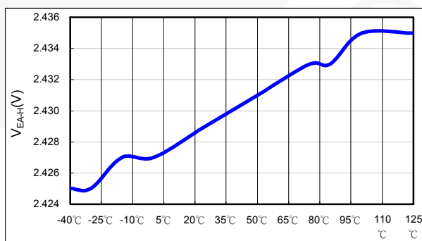
Figure 39. V_{\text{EA-H}} vs. Temperature
