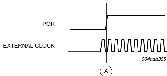
Fig 4. External clock with respect to power-on reset
