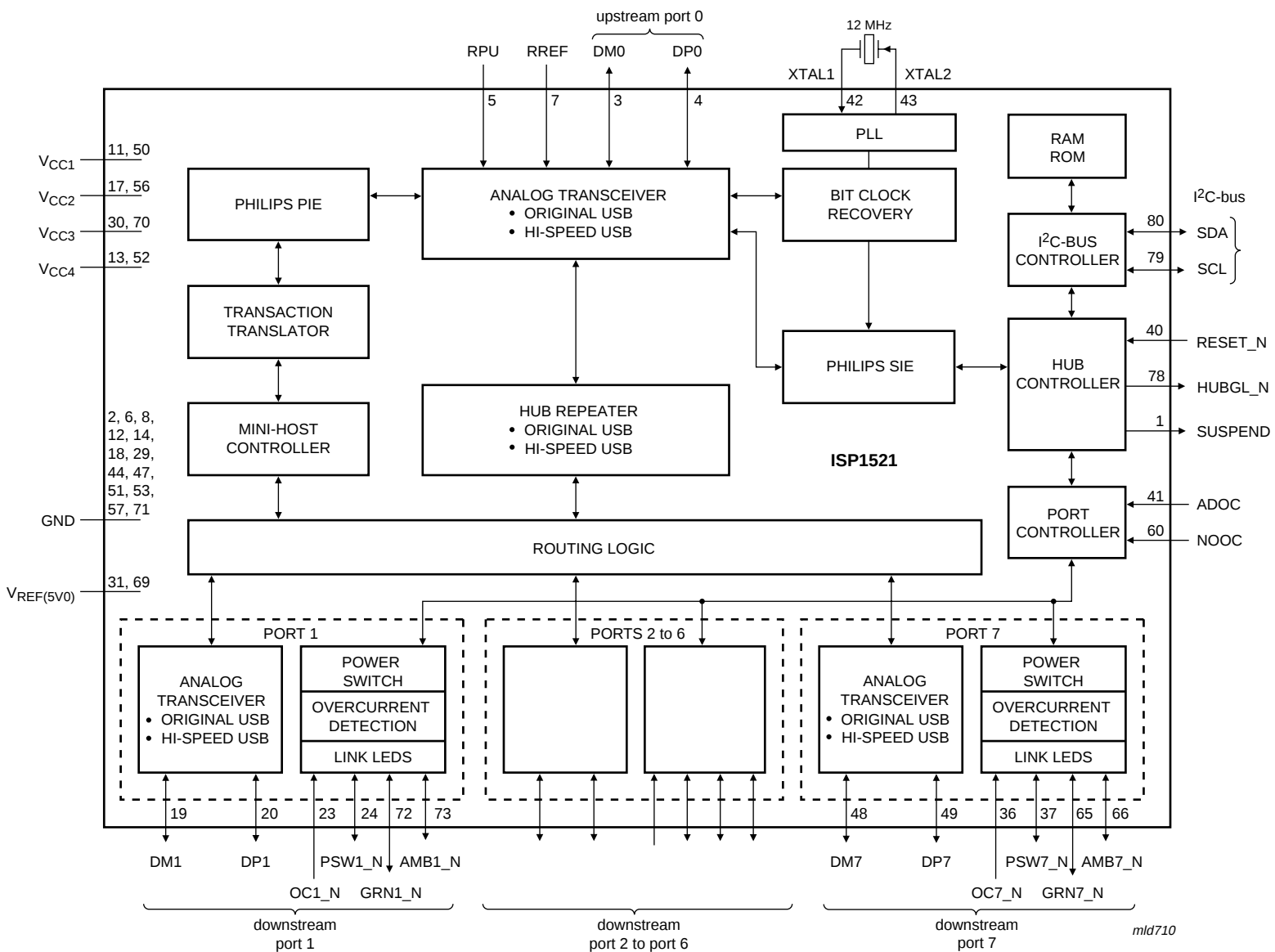
Fig 1. Block diagram
