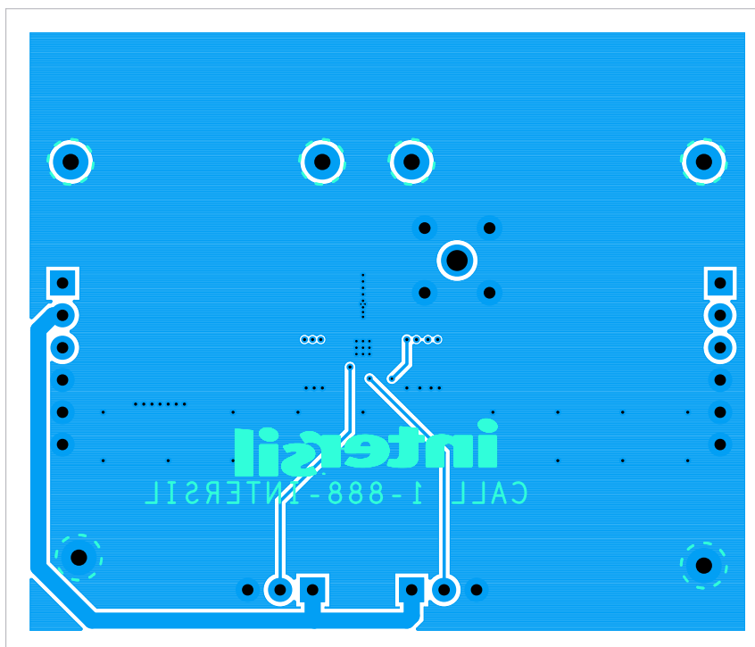
FIGURE 9. BOTTOM LAYER
