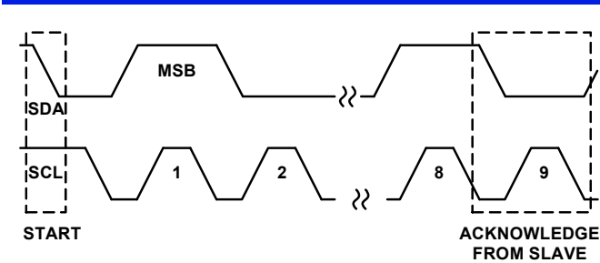
FIGURE 23. ACKNOWLEDGE ON THE SMBus
