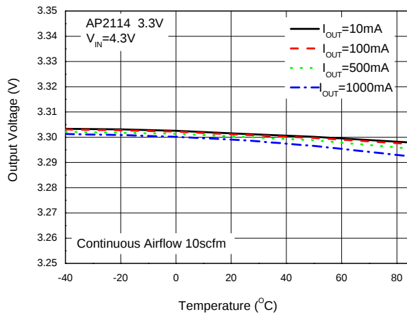
Figure 19. Output Voltage vs. Temperature
