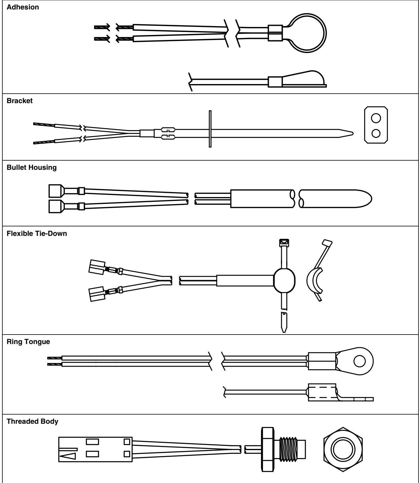
Figure 1. Mounting Methods
