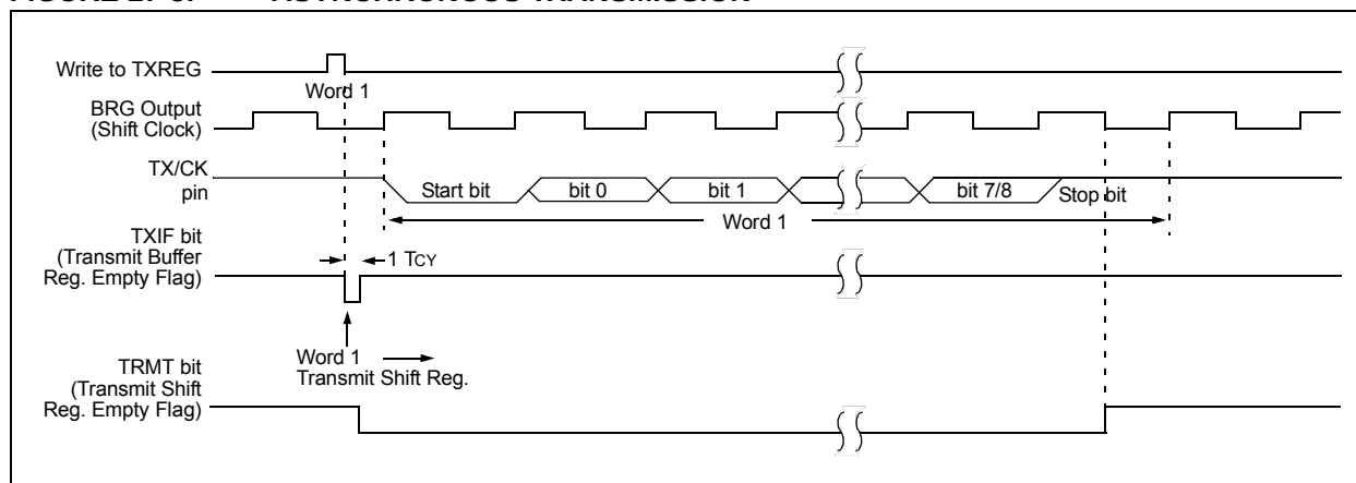
FIGURE 27-3: ASYNCHRONOUS TRANSMISSION
