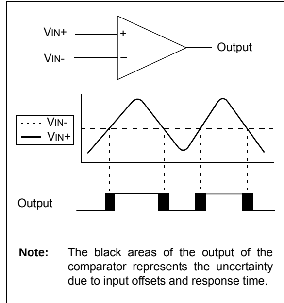
FIGURE 20-1: SINGLE COMPARATOR
