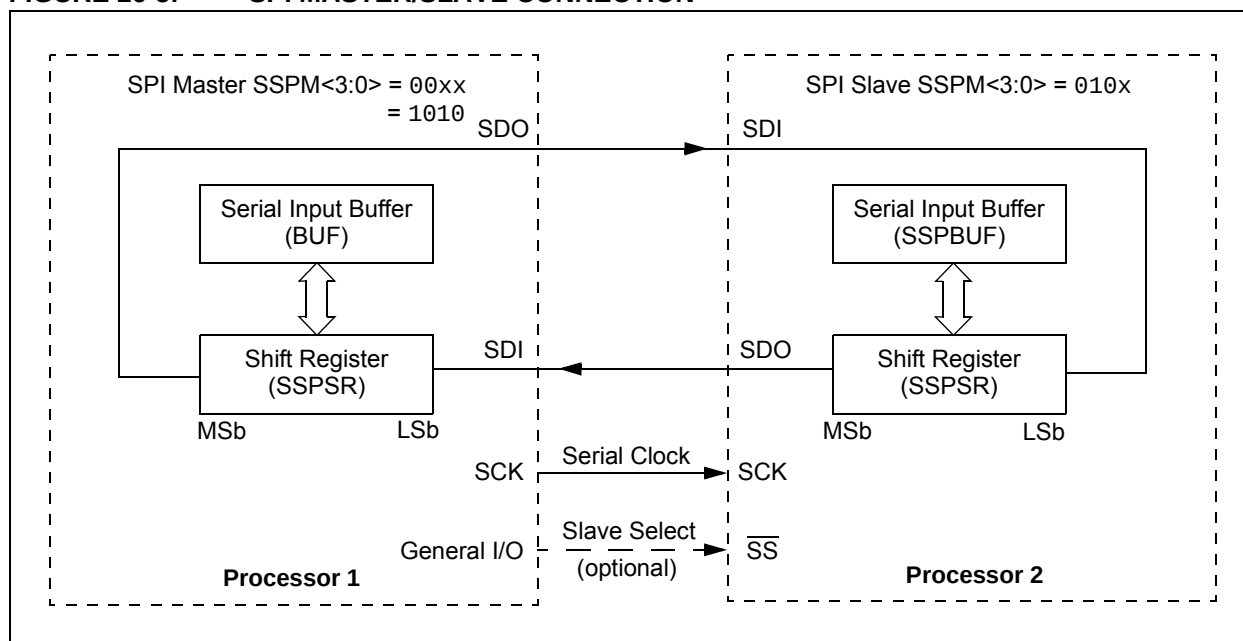
FIGURE 26-5: SPI MASTER/S�AVE CONNECTION
