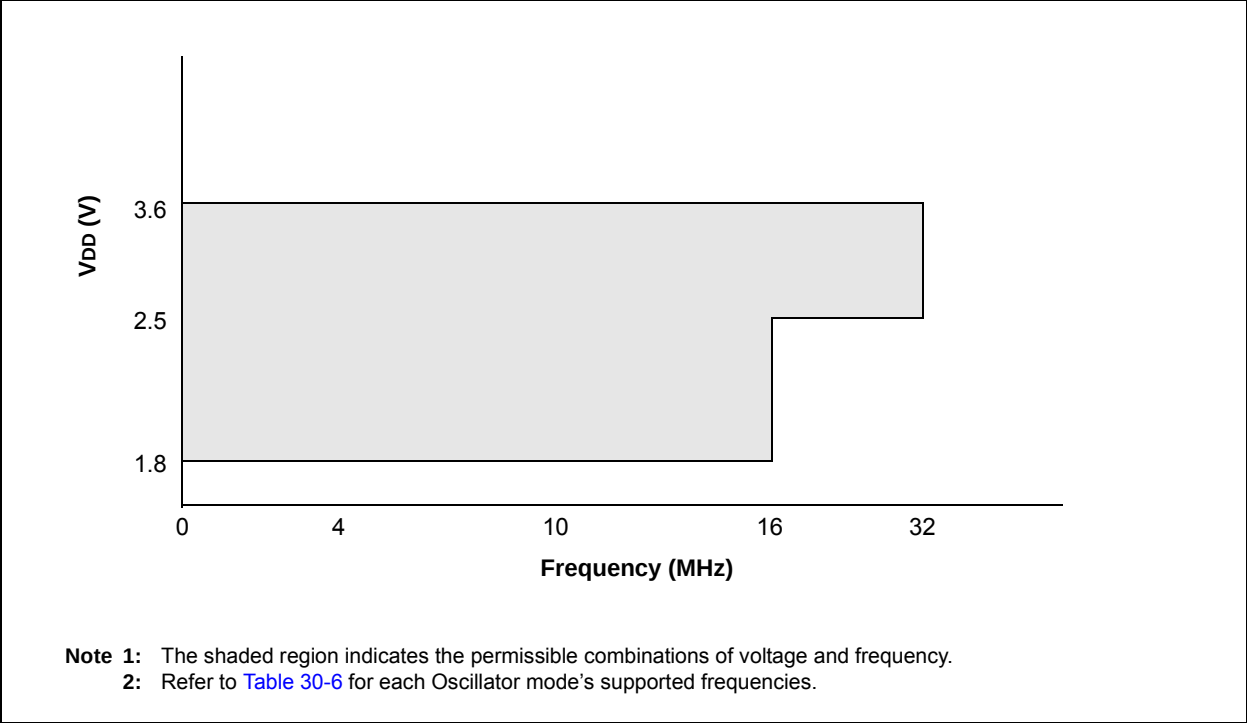
FIGURE 30-2: PIC16LF1784/6/7 VOLTAGE FREQUENCY GRAPH, -40^{\circ}\text{C} \leq \text{Ta} \leq +125^{\circ}\text{C}
