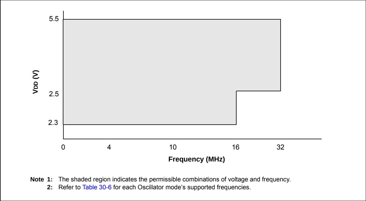
FIGURE 30-1: PIC16F1784/6/7 VOLTAGE FREQUENCY GRAPH, -40^{\circ}\text{C} \leq \text{Ta} \leq +125^{\circ}\text{C}
