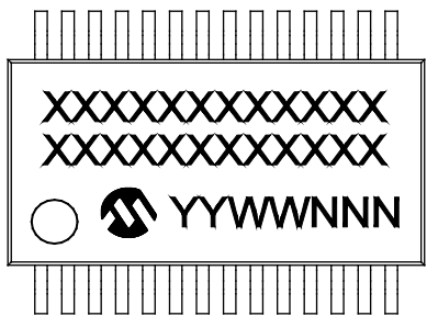
28-Lead SSOP (5.30 mm)
