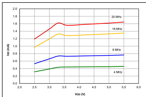
FIGURE 31-29: I_{DD} Typical, HS Oscillator, 25^\circ\text{C} , PIC16F1784/6/7 Only.
