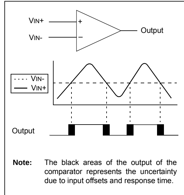
FIGURE 20-1: SINGLE COMPARATOR
