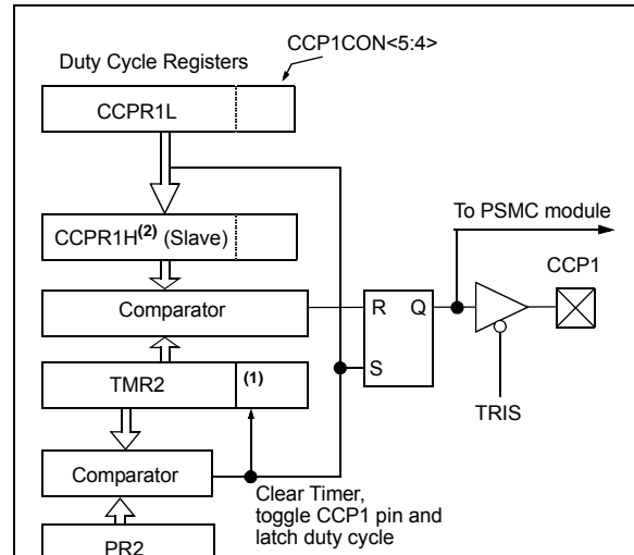
FIGURE 25-4: SIMPLIFIED PWM BLOCK DIAGRAM
