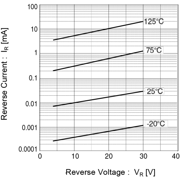
Fig.12 Reverse Current vs. Reverse Voltage
