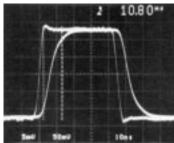
RISE TIME = 10.8ns, PROPAGATION DELAY = 6ns LT1194 • TPC20
