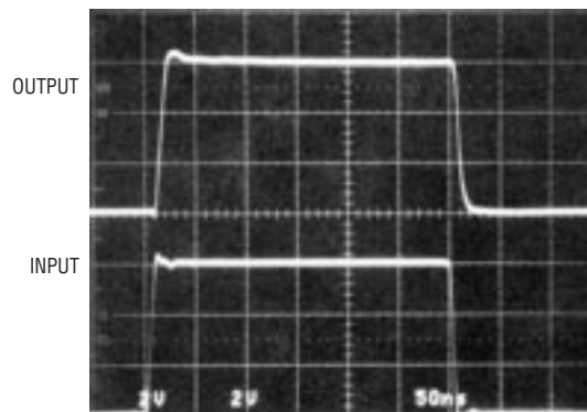
20dB INPUT OVERDRIVE, V_C = -4.2V LT1194 • TA04
