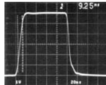
R_L = 150\Omega , +SR = 430V/ \mu s, -SR = 500V/ \mu s LT1194 • TPC21
