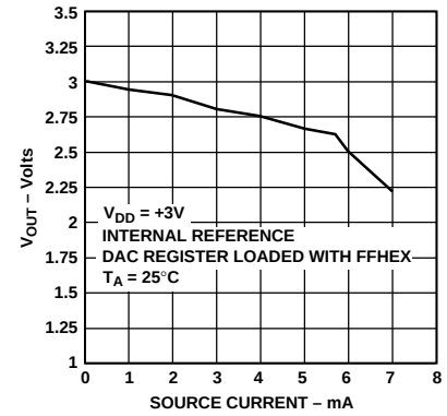
Figure 5. Output Source Current Capability with V_{DD} = 3 V
