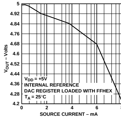
Figure 4. Output Source Current Capability with V_{DD} = 5 V
