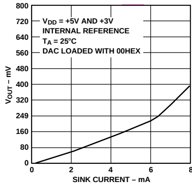
Figure 3. Output Sink Current Capability with V_{DD} = 3 V and V_{DD} = 5 V
