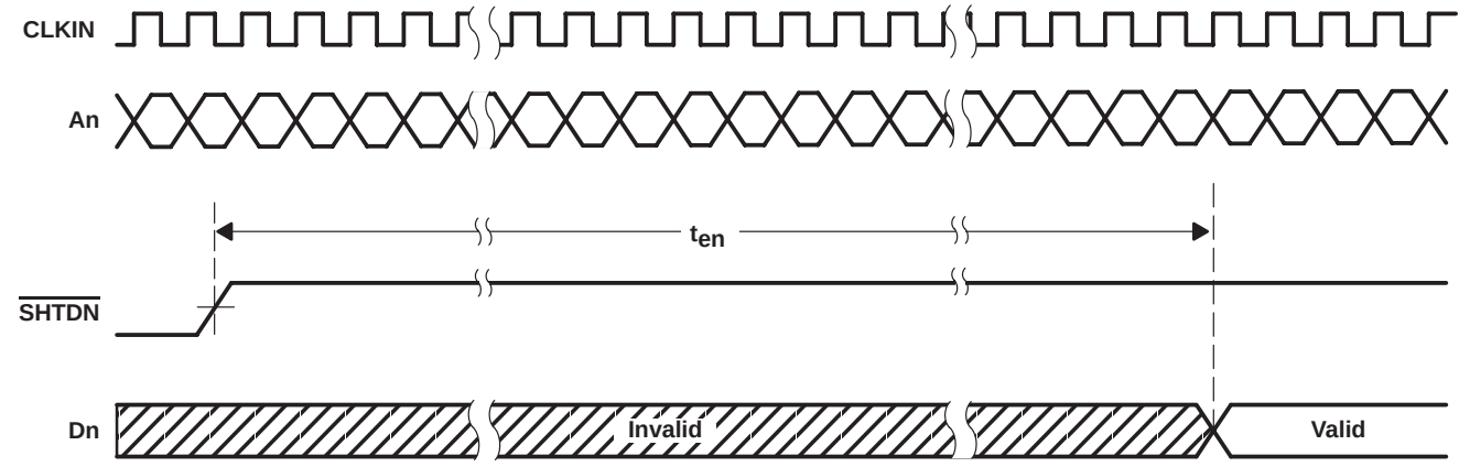
Figure 9. Enable Time
