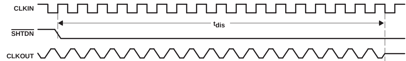
Figure 10. Disable Time
