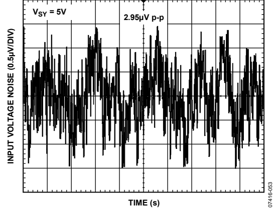
Figure 47. Input Voltage Noise, 0.1 Hz to 10 Hz Noise
