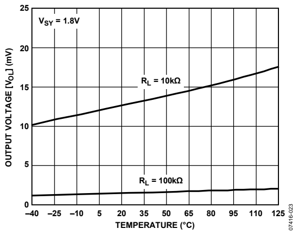
Figure 21. Output Voltage ( V_{O} ) vs. Temperature
