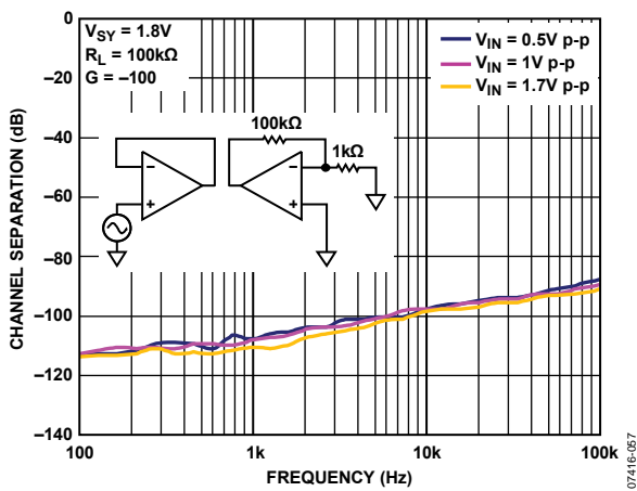
Figure 45. Channel Separation vs. Frequency
