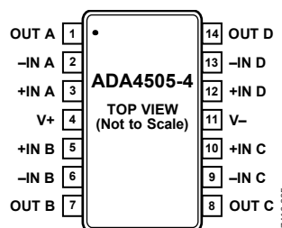
Figure 5. 14-Lead TSSOP (RU-14)
