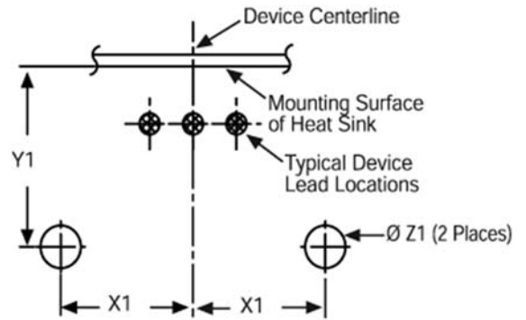
Mounting Details:
