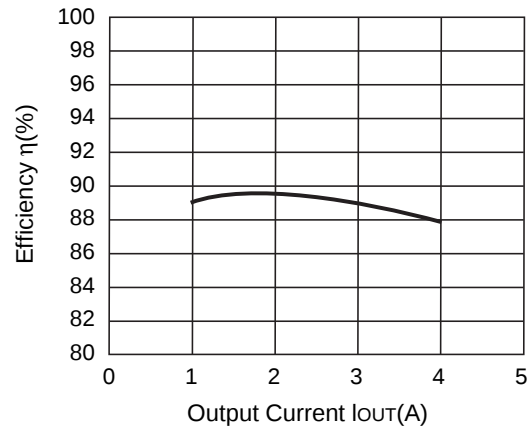
R1224N332M ( V_{IN}=10V )
