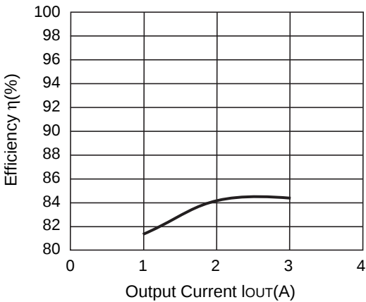
R1224N332M ( V_{IN}=18V )
