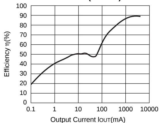
R1224N502G ( V_{IN}=16V )
