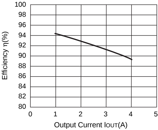
R1224N332M ( V_{IN}=5V )
