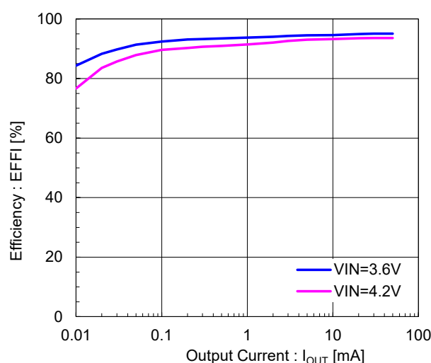
XCL210B301GR-G (V OUT =3.0V)
