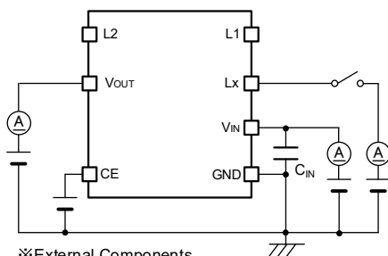
< Circuit No.③ >
