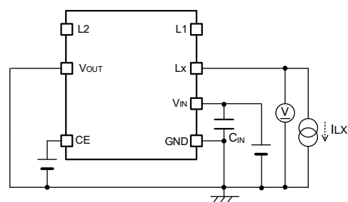
< Circuit No.⑥ >
