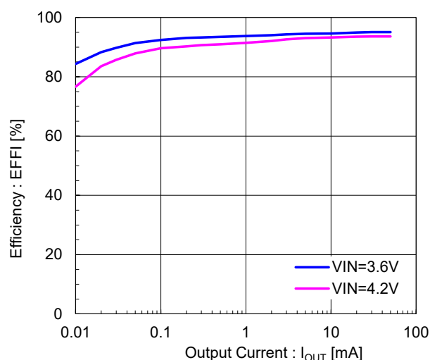
XCL210B301GR-G ( V_{OUT}=3.0V )
