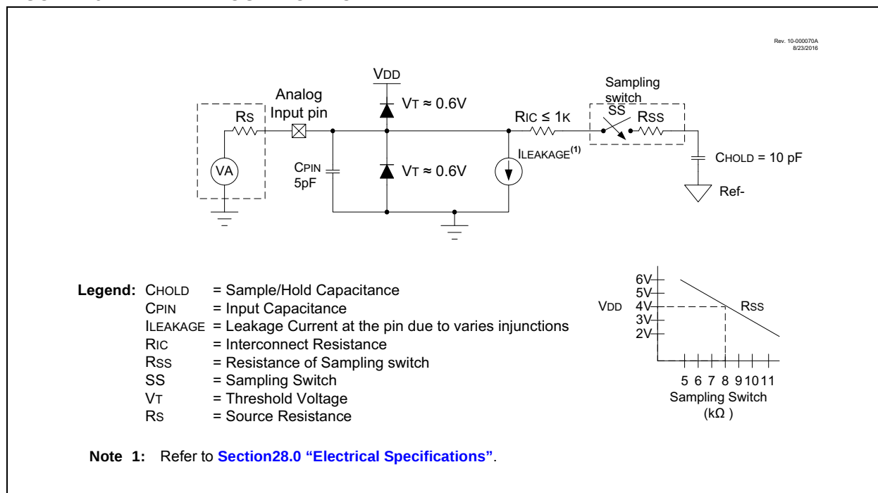
FIGURE 16-4: ANALOG INPUT MODEL
