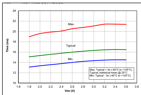
FIGURE 29-46: WDT Time-Out Period, PIC12LF1612/16F1613 Only.
