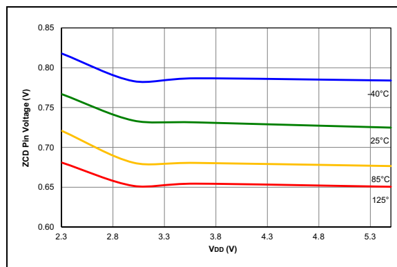
FIGURE 29-99: ZCD Pin Voltage, Typical Measured Values.
