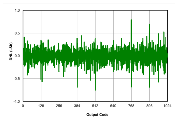
FIGURE 29-63: ADC 10-bit Mode, Single-Ended DNL, V_{DD} = 3.0V , T_{AD} = 1\text{ }\mu\text{S} , 25^\circ\text{C} .
