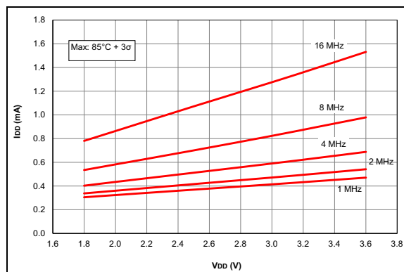
FIGURE 29-18: I_{DD} Maximum, HFINTOSC Mode, PIC12LF1612/16F1613 Only.
