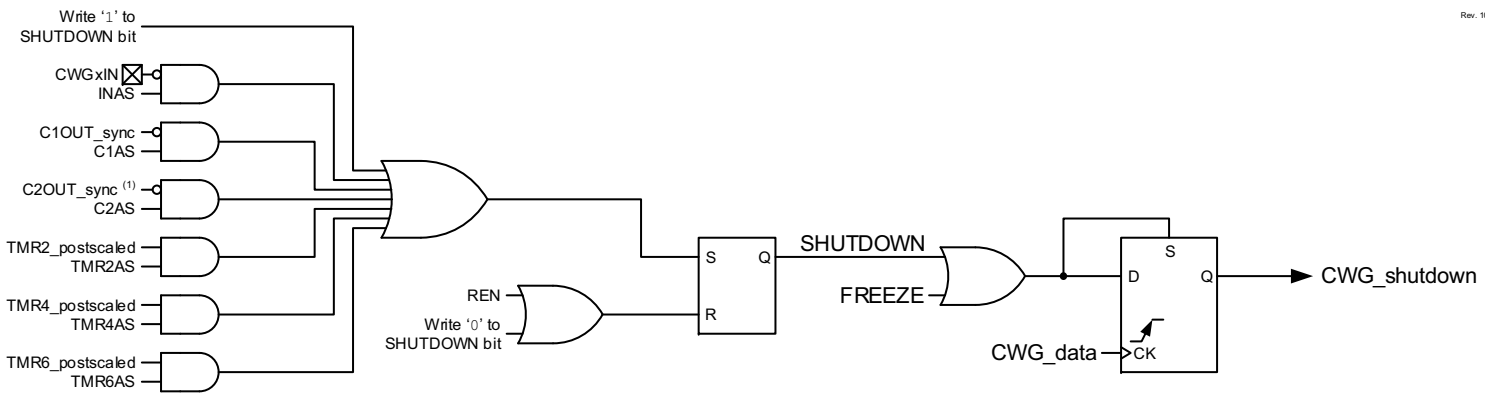
FIGURE 24-12: CWG SHUTDOWN BLOCK DIAGRAM
