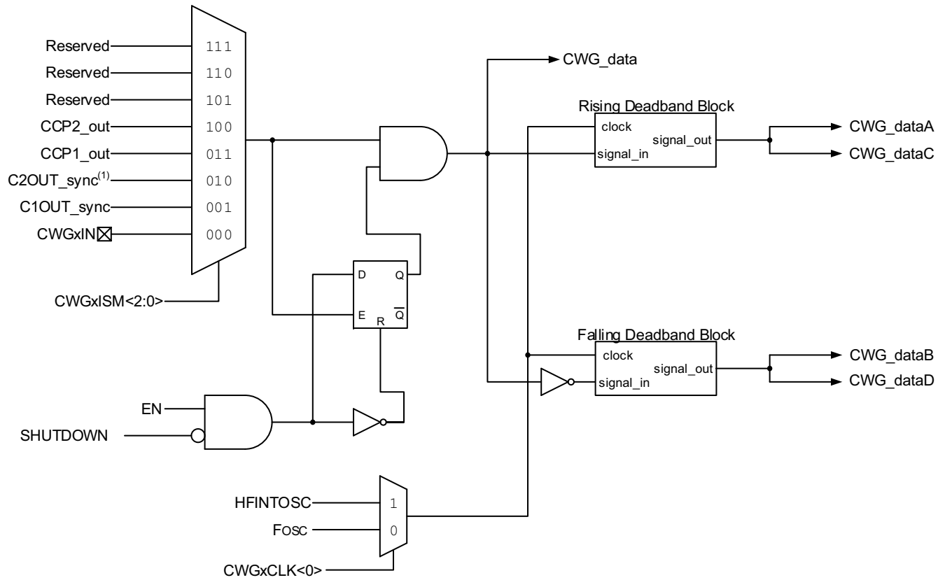
FIGURE 24-1: SIMPLIFIED CWG BLOCK DIAGRAM (HALF BRIDGE MODE)
