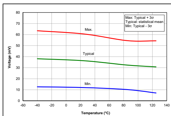
FIGURE 29-52: Brown-Out Reset Hysteresis, High Trip Point (BORV = 0).
