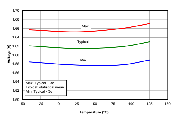
FIGURE 29-57: POR Release Voltage.
