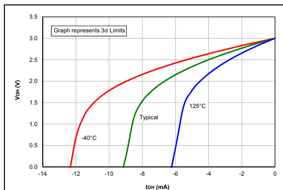
FIGURE 29-39: V_{OH} vs. I_{OH} Over Temperature, V_{DD} = 3.0V .
