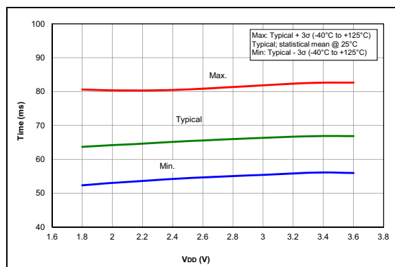
FIGURE 29-56: PWRT Period, PIC12LF1612/16F1613 Only.
