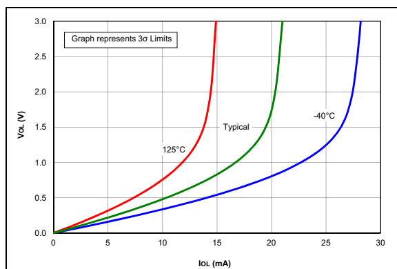
FIGURE 29-40: V_{OL} vs. I_{OL} Over Temperature, V_{DD} = 3.0V .
