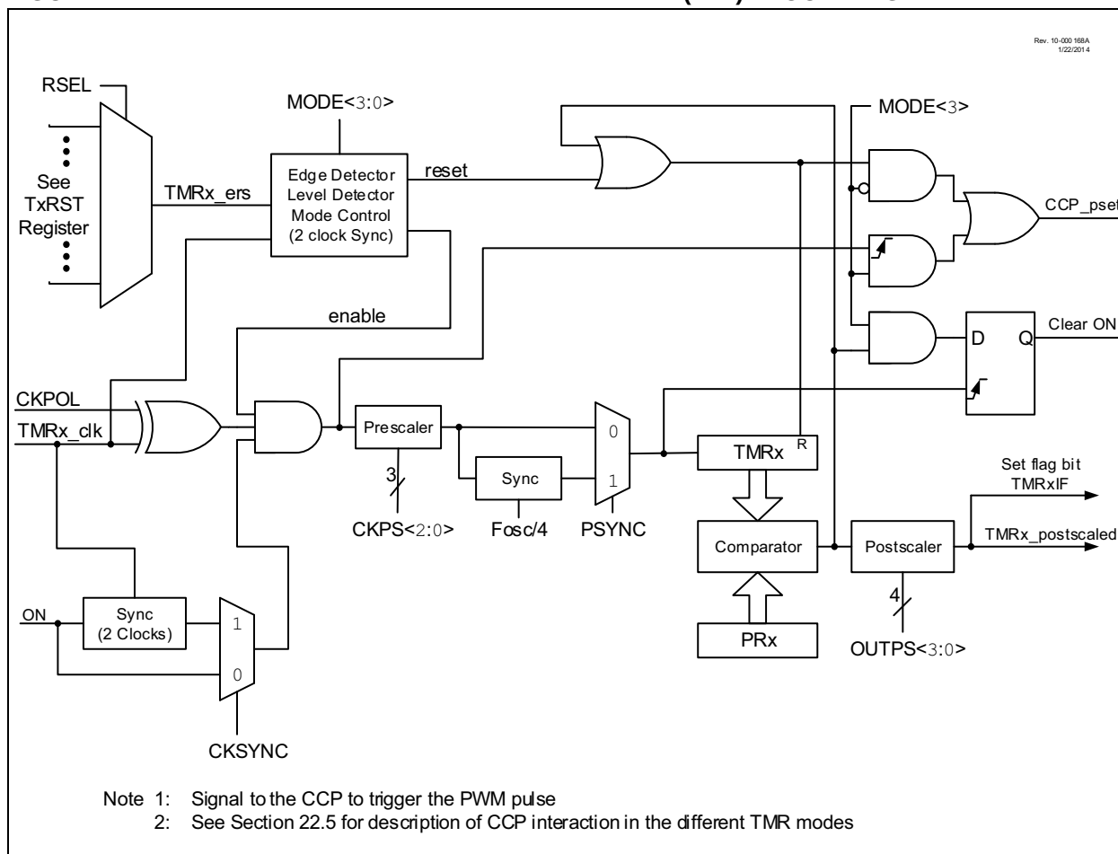
FIGURE 22-1: TIMER2 WITH HARDWARE LIMIT TIMER (HLT) BLOCK DIAGRAM
