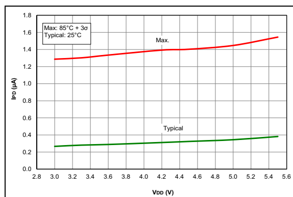
FIGURE 29-30: I_{PD} , LP Brown-Out Reset (LPBOR = 0), PIC12F1612/16F1613 Only.
