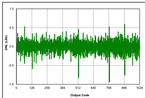
FIGURE 29-64: ADC 10-bit Mode, Single-Ended DNL, V_{DD} = 3.0V , T_{AD} = 4\text{ }\mu\text{S} , 25^\circ\text{C} .
