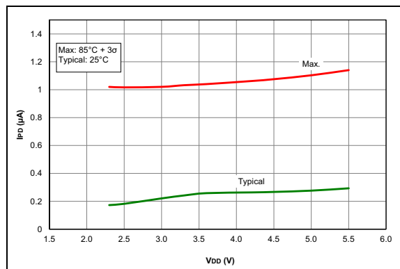
FIGURE 29-34: I_{PD} , ADC Non-Converting, PIC12F1612/16F1613 Only.
