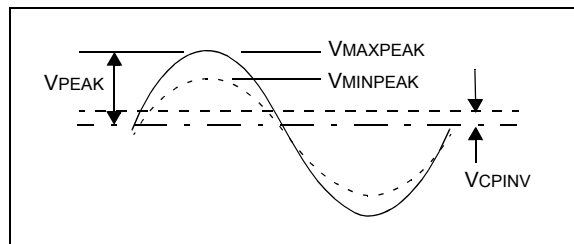
FIGURE 19-1: EXTERNAL VOLTAGE
