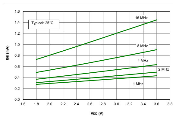
FIGURE 29-17: I_{DD} Typical, HFINTOSC Mode, PIC12LF1612/16F1613 Only.
