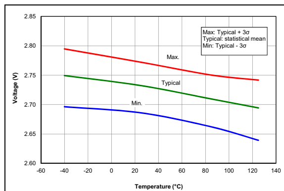
FIGURE 29-51: Brown-Out Reset Voltage, High Trip Point (BORV = 0).
