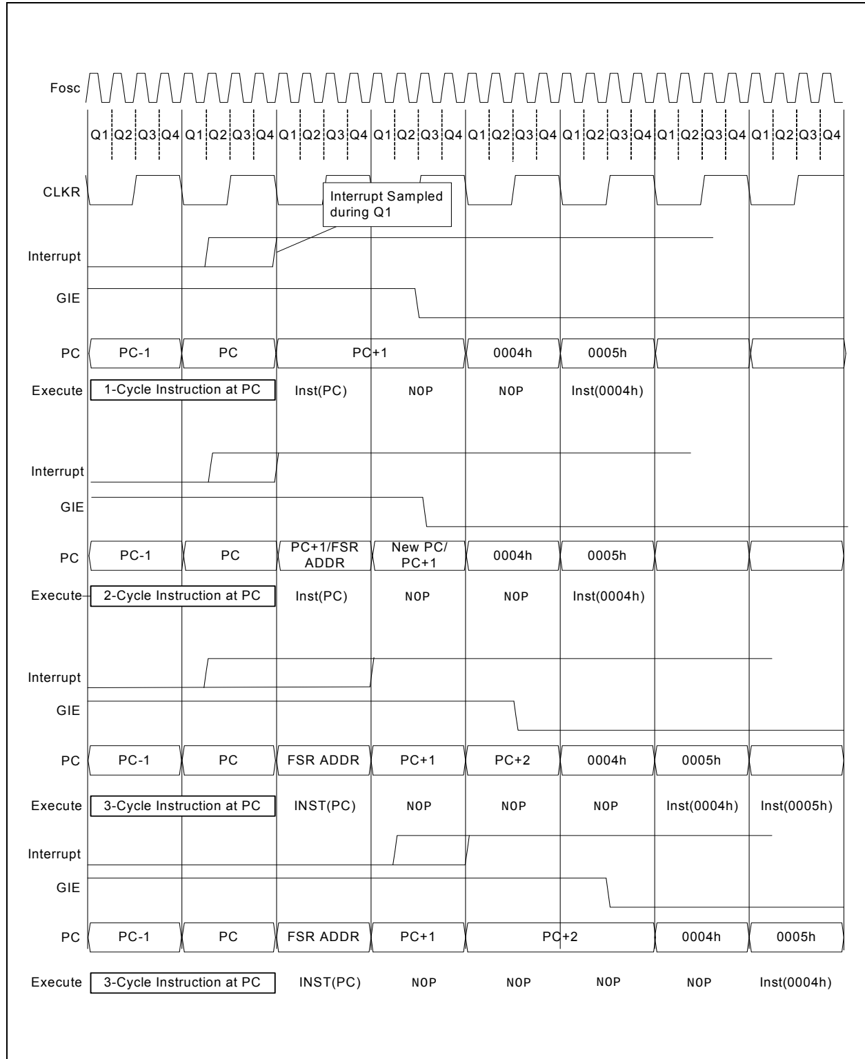
FIGURE 7-2: INTERRUPT LATENCY
