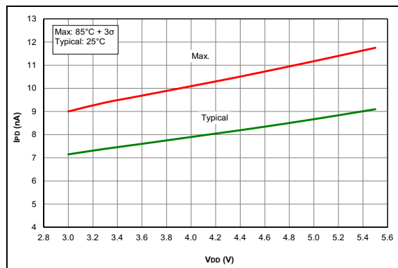
FIGURE 29-28: I_{PD} , Brown-Out Reset (BOR), BORV = 1, PIC12F1612/16F1613 Only.
