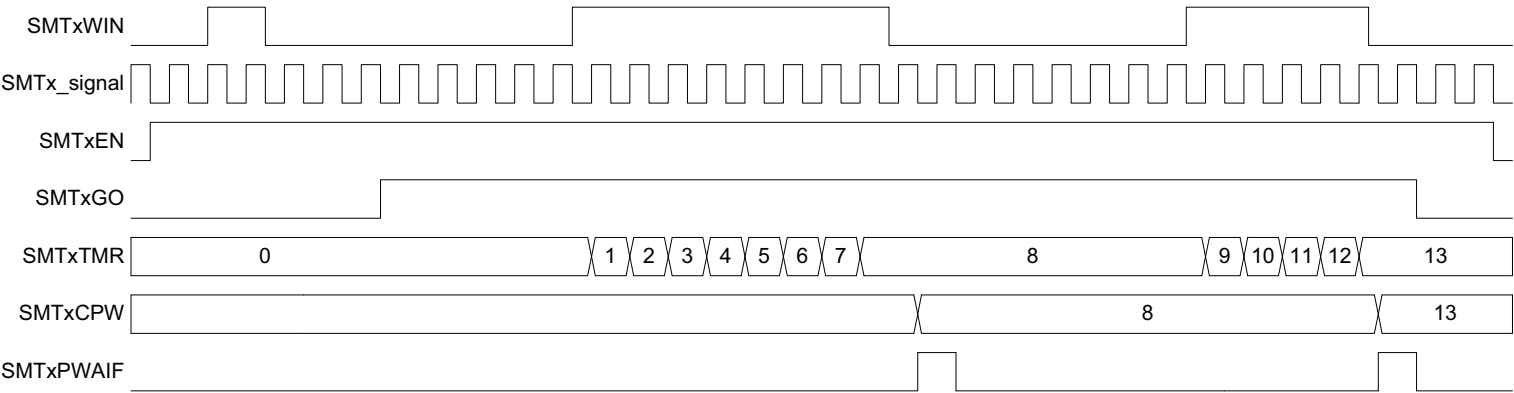
FIGURE 25-20: GATED COUNTER MODE SINGLE ACQUISITION TIMING DIAGRAM
