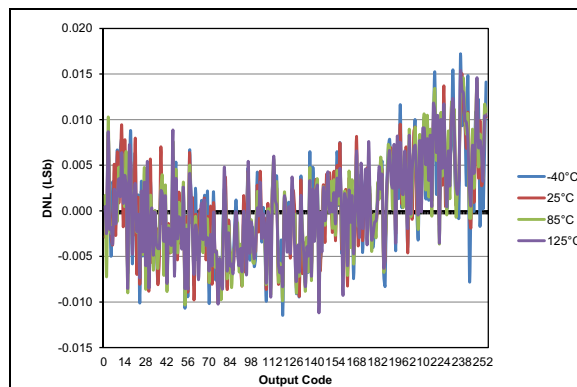
FIGURE 29-92: Typical DAC INL Error, V_{DD} = 5.0V , V_{REF} = \text{External } 5V , PIC12F1612/16F1613 Only.
