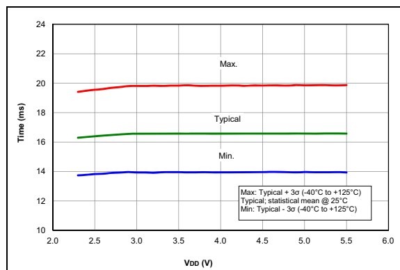
FIGURE 29-45: WDT Time-Out Period, PIC12F1612/16F1613 Only.
