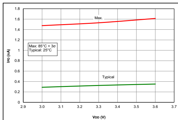
FIGURE 29-29: I_{PD} , LP Brown-Out Reset (LPBOR = 0), PIC12LF1612/16F1613 Only.
