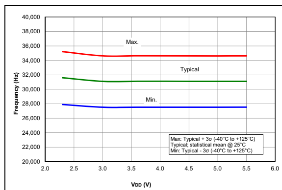
FIGURE 29-44: LFINTOSC Frequency, PIC12F1612/16F1613 Only.
