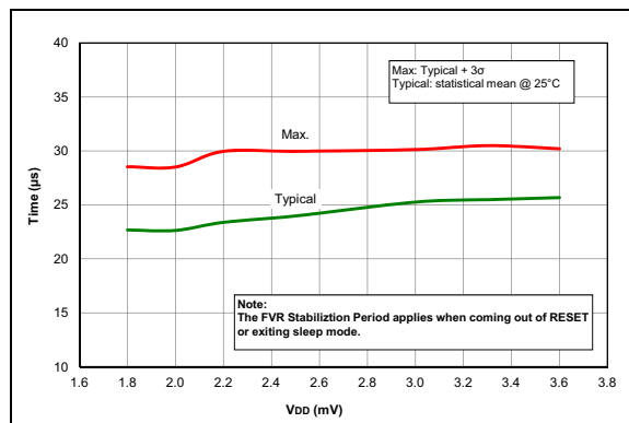
FIGURE 29-62: FVR Stabilization Period, PIC12LF1612/16F1613 Only.
