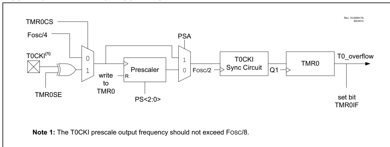
FIGURE 20-1: TIMER0 BLOCK DIAGRAM
