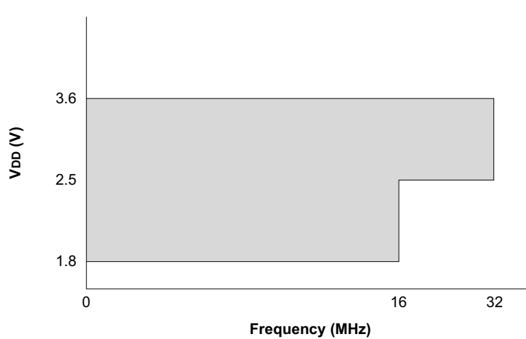
FIGURE 28-2: VOLTAGE FREQUENCY GRAPH, -40^{\circ}\text{C} \leq T_A \leq +125^{\circ}\text{C} , PIC12LF1612/16F1613 ONLY
